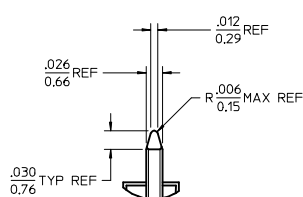
DETAIL Y SCALE 5:1 SEE NOTE 10
