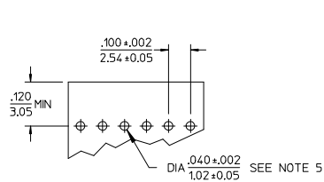
KINKED PIN OPTION SEE NOTE 5
