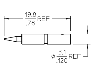
CONTACT
