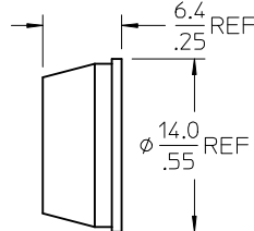
SLEEVE
