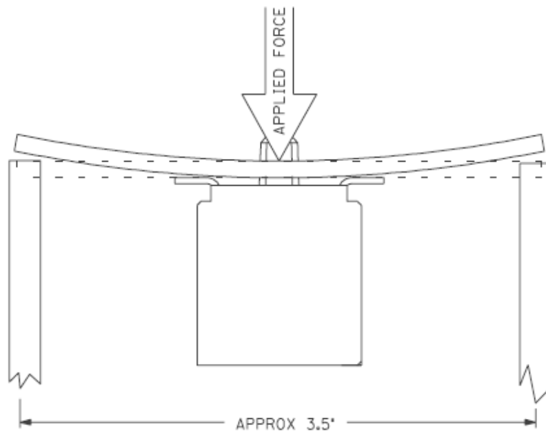
FIGURE 6 PARALLEL SOLDER JOINT FATIGUE (TENSION)
