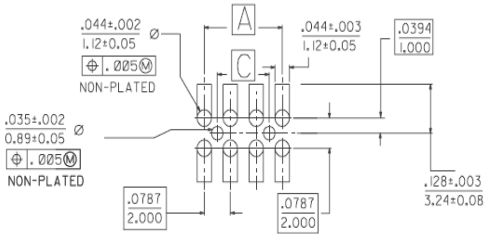
BOTTOM ENTRY LAND LAYOUT
