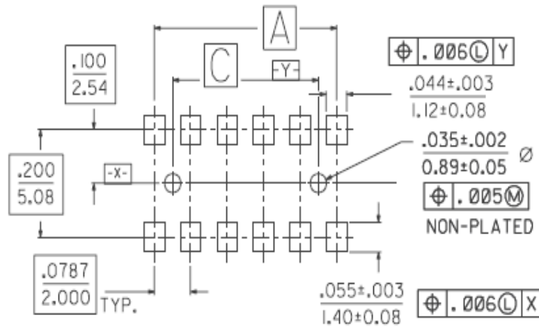
SMT PC BOARD LAND LAYOUT
