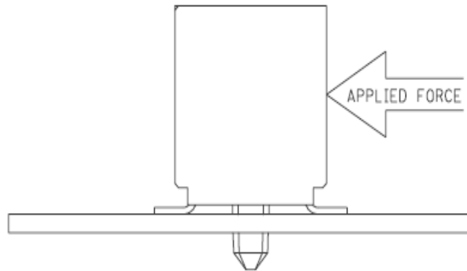
FIGURE 4 PERPENDICULAR SHEAR
