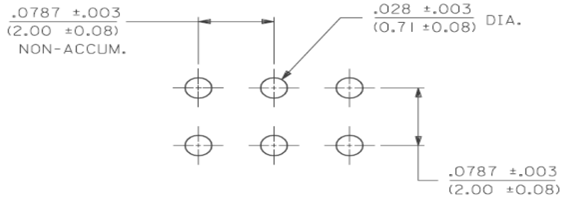
FIGURE 1 RECOMMENDED P.C. BOARD HOLE LAYOUT
