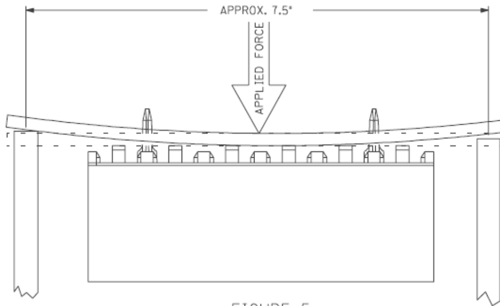
FIGURE 5 PERPENDICULAR SOLDER JOINT FATIGUE (TENSION)
