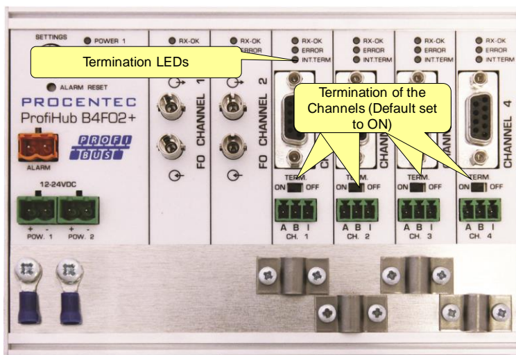
Fig. 15 - Termination switches
