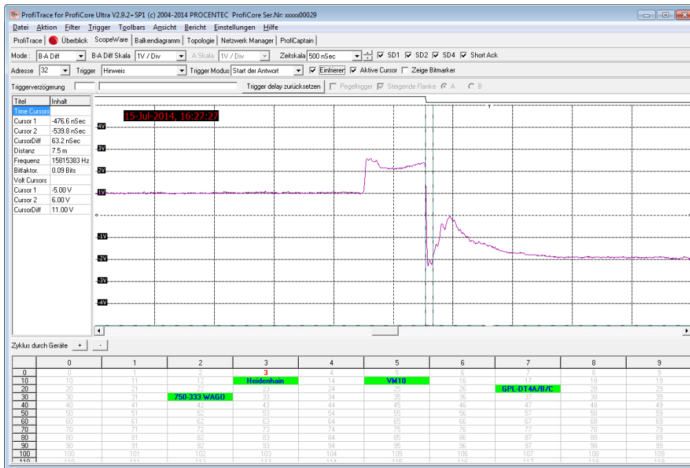
Abb. 39 - Kurzschluss (B-Schild) Diff
